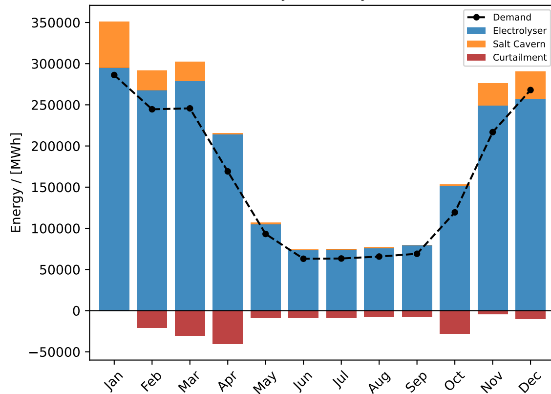
Hydrogen Bus Monthly Flexibility Stack
