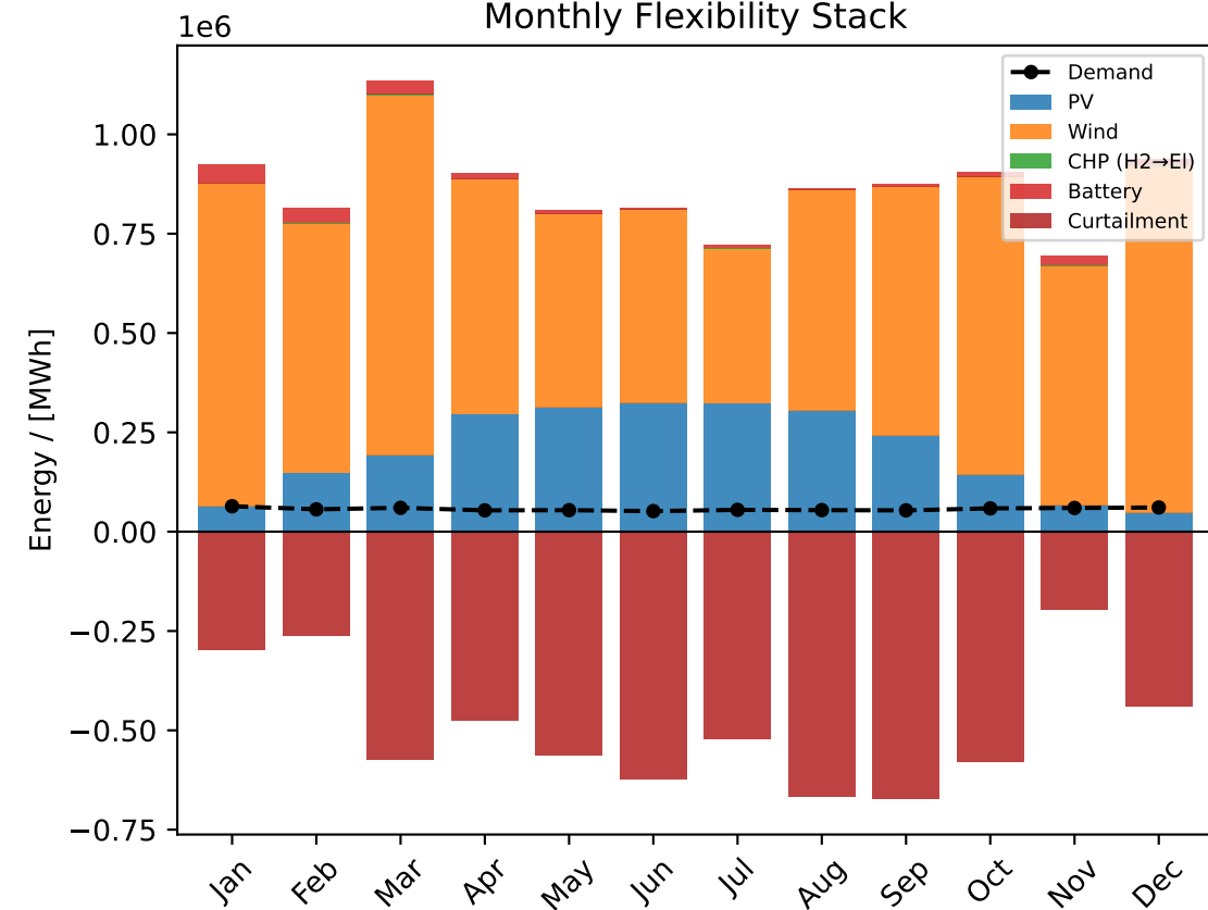
Electricity Bus Net Monthly Flexibility
