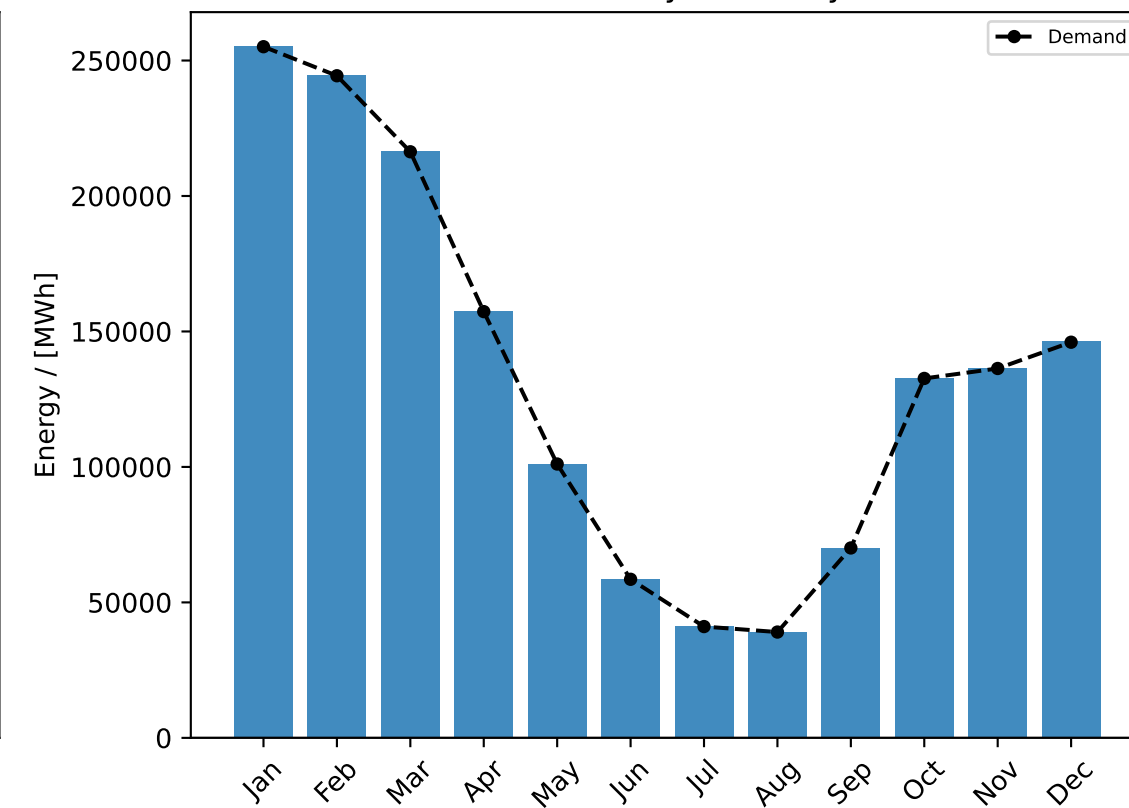
Heat Bus Net Monthly Flexibility
