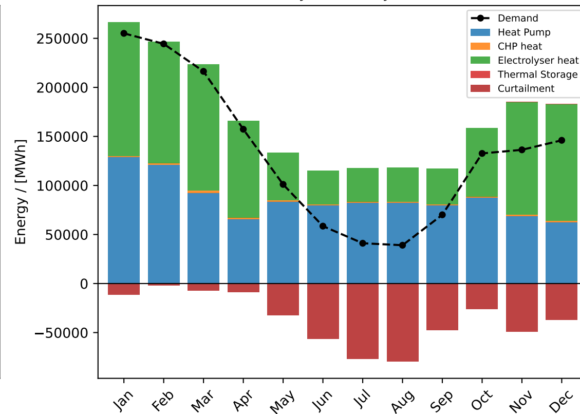
Heat Bus Monthly Flexibility Stack
